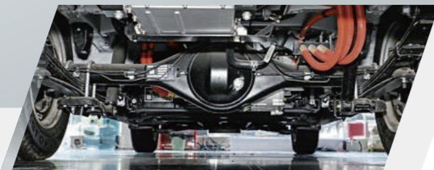
4 steel leaf springs in rear + Load-bearing rear axle, with a load capacity up to 1.2T
